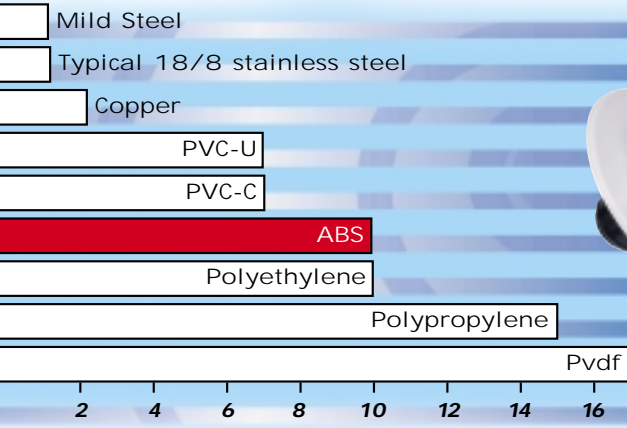
Thermal Coefficient of Linear Expansion for Various Materials
